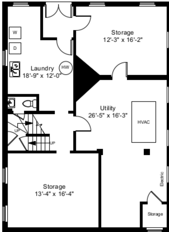
Basement Plan Ceiling Height = 7'-8"
